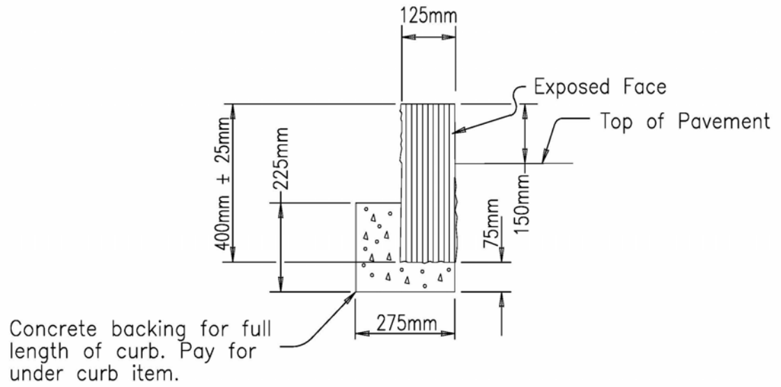
Item 609.0301M SAWED OR HAMMERED TOP, QUARRY SPLIT FACE DETAIL OF GRANITE CURB – TYPE A Not to Scale
